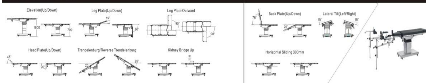
Movements Diagram of ET300C
